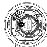
With grille: Ø257mm Without grille: Ø247mm Hole Cut: Ø220mm
